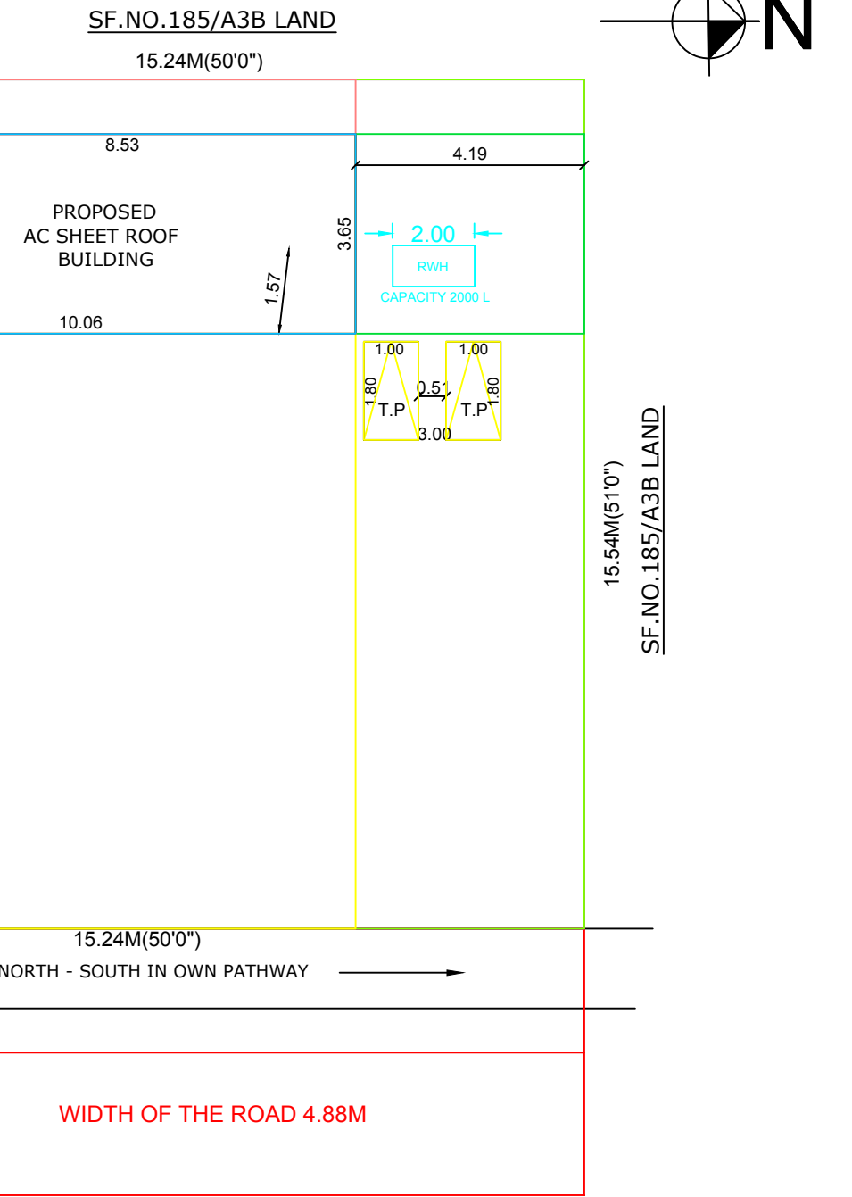
SITE PLAN - MEANT FOR FARM HOUSE
