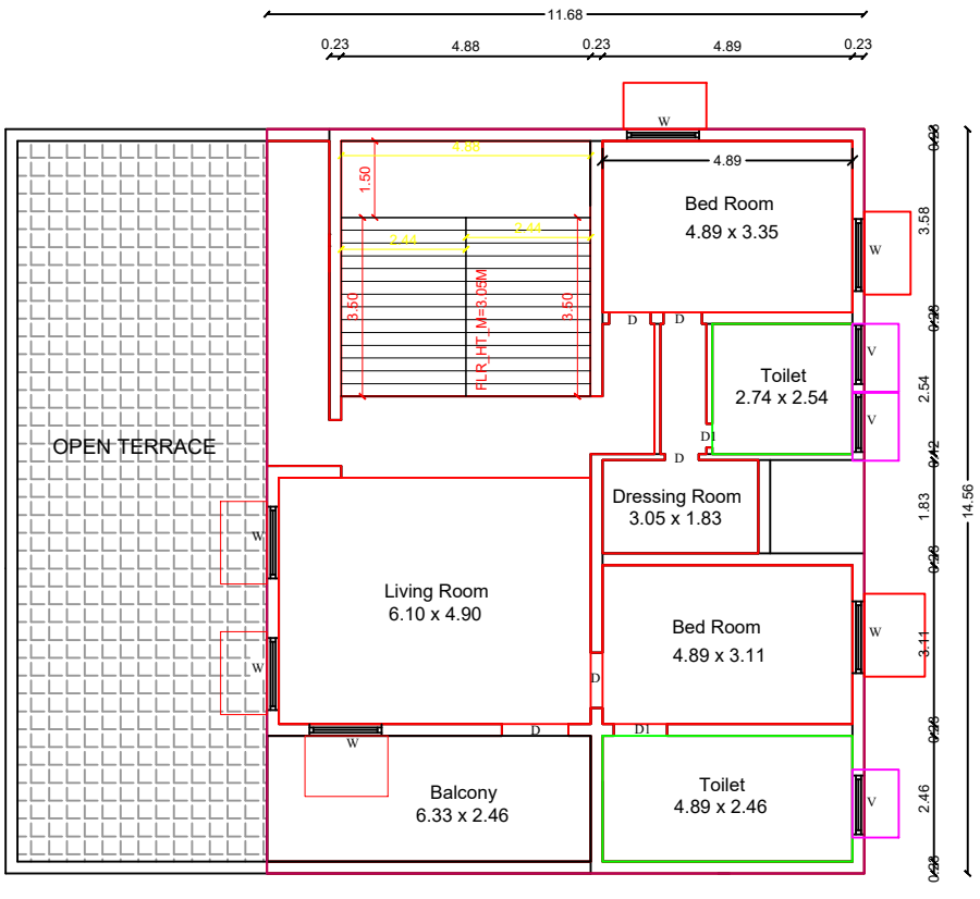
FIRST FLOOR BUILDING
