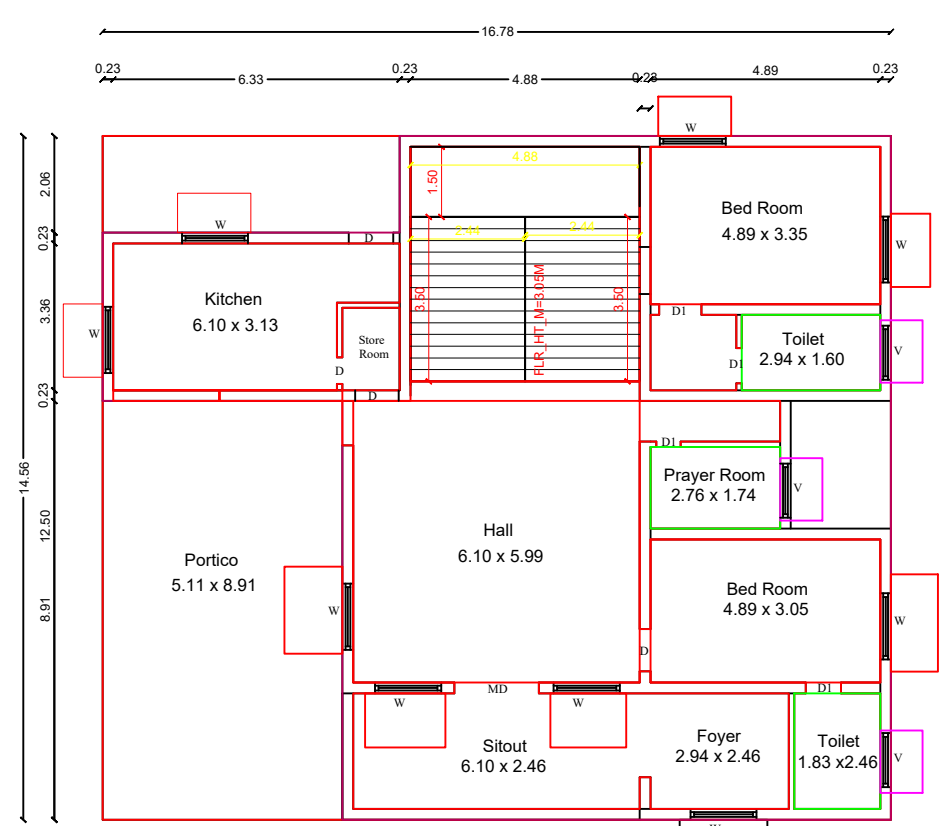
GROUND FLOOR BUILDING
