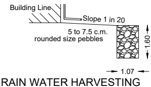
RAIN WATER HARVESTING
