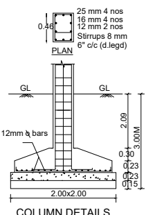
COLUMN DETAILS
