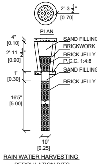
RAIN WATER HARVESTING PERCOLATION PITS
