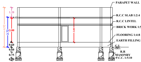
"SECTION 'AB'"
