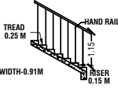
STAIRCASE DETAILS
