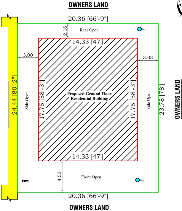
SITE PLAN
