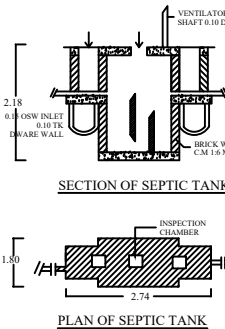
SEPTIC TANK
