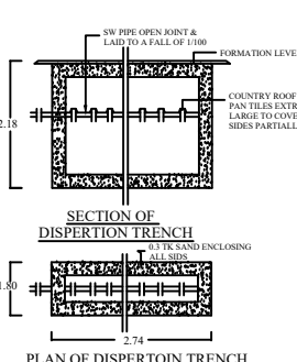
DISPERSION TRENCH
