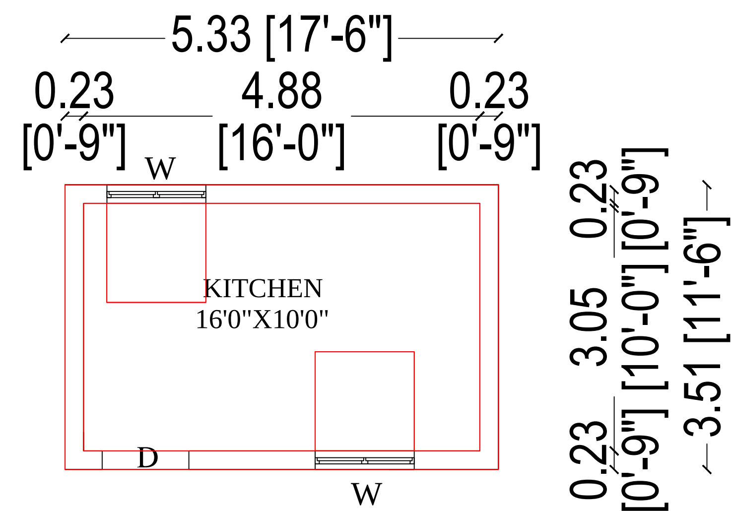
PROPOSED PLAN
