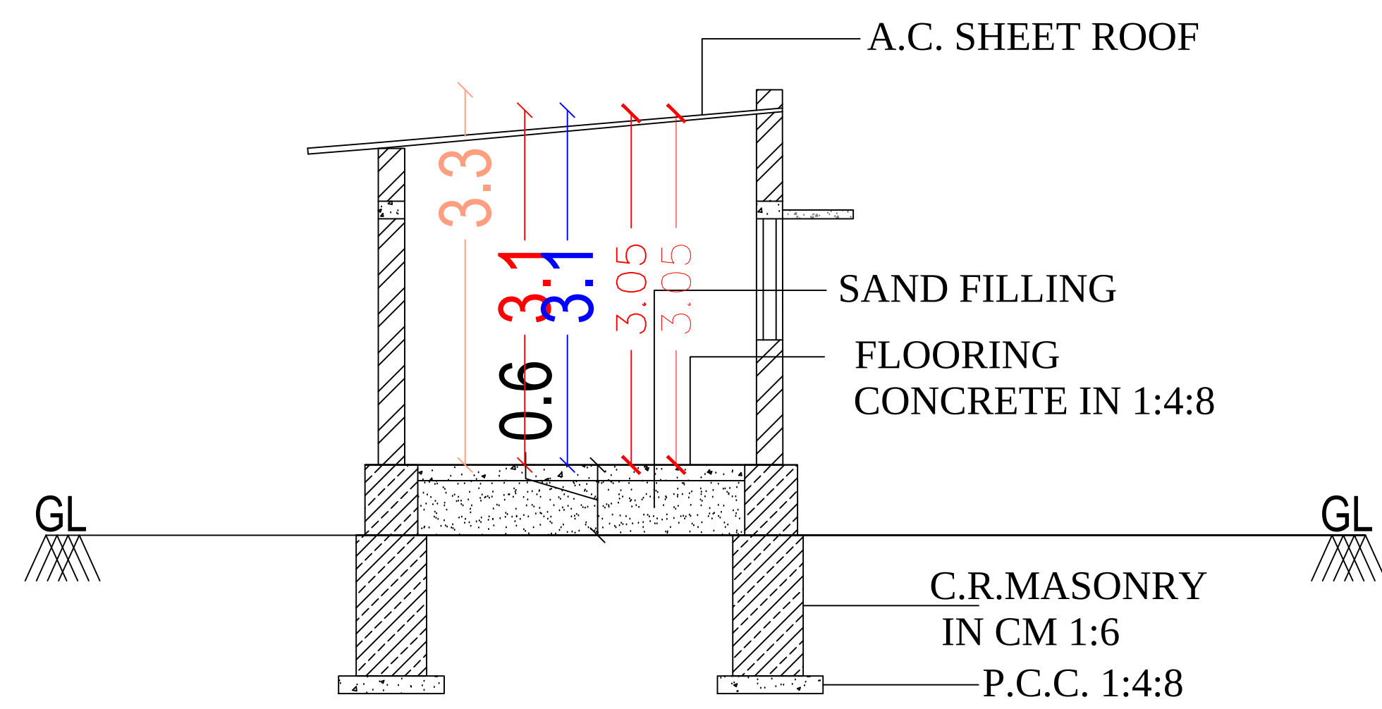
SECTION
