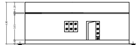
ELEVATION FACING NORTH
