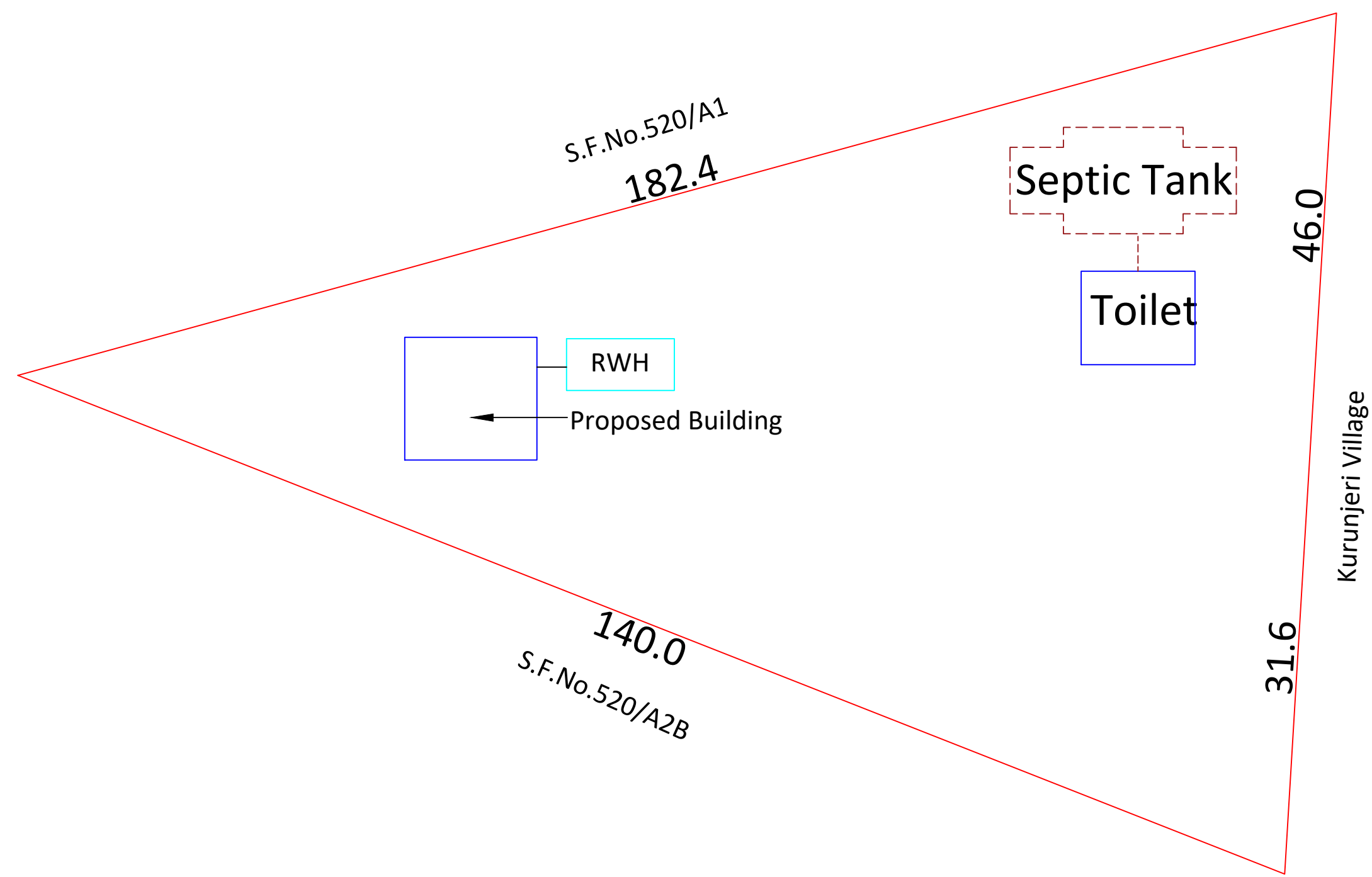
SITE PLAN
