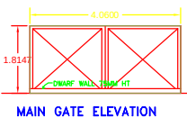
MAIN GATE ELEVATION
