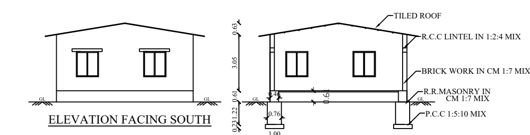
ELEVATION FACING SOUTH
