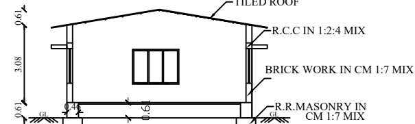
SECTION ON BB'
