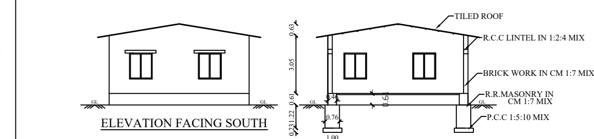
ELEVATION FACING SOUTH
