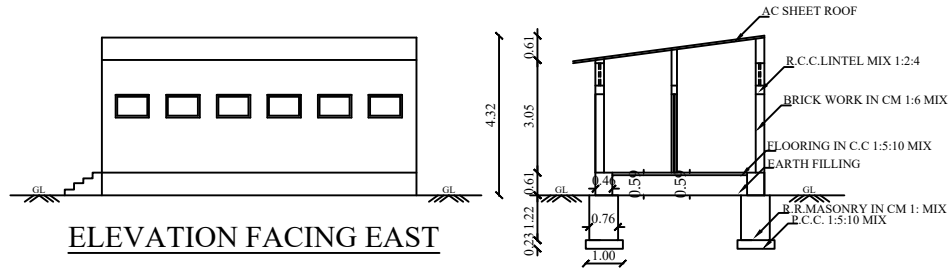
ELEVATION FACING EAST
