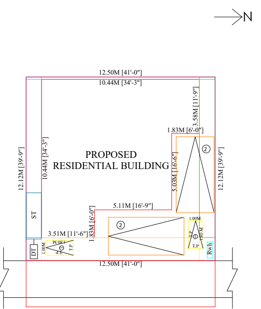
SITE PLAN(MEANT FOR CONSTRUCTION)
