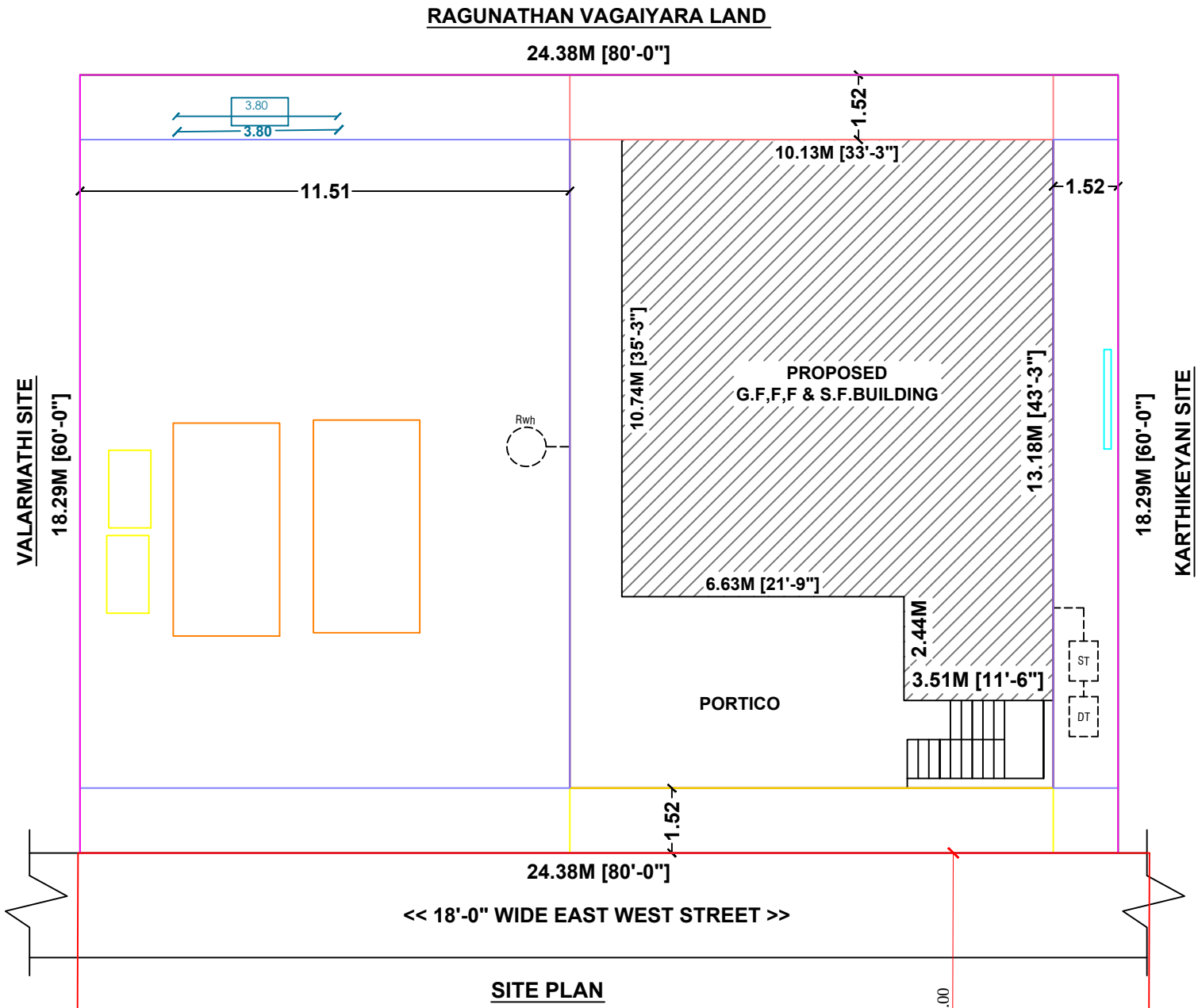
SITE PLAN
