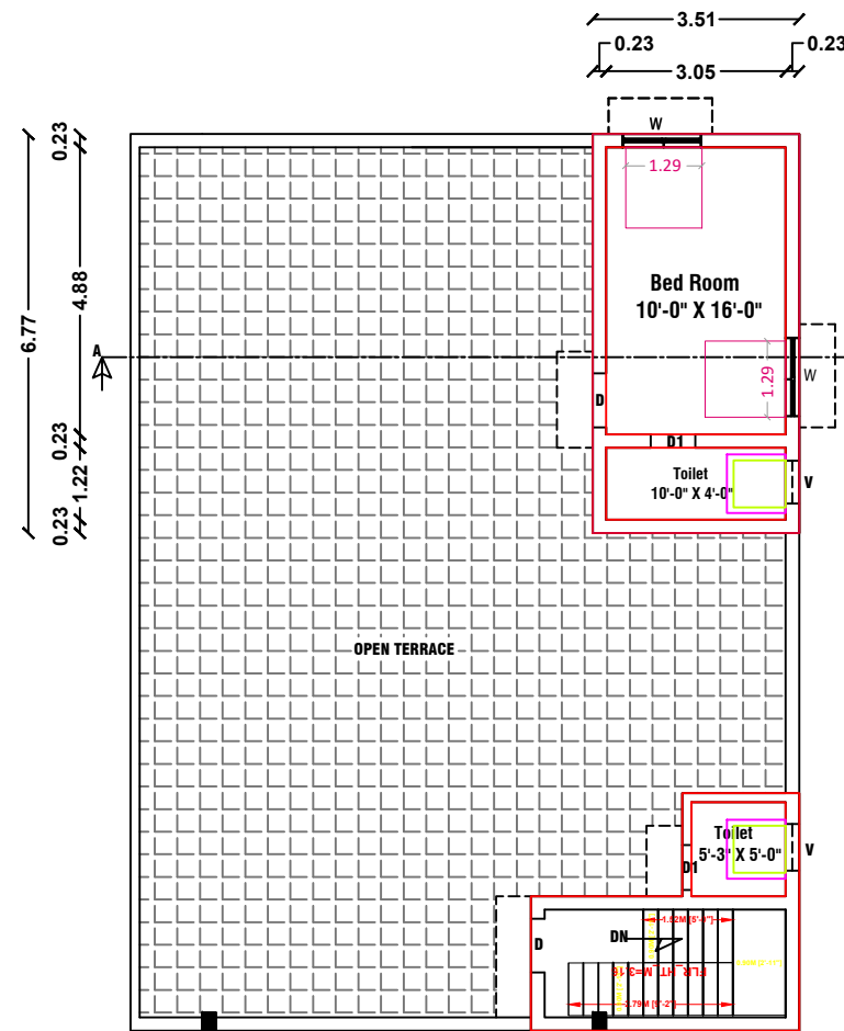
PRO.SECOND FLOOR PLAN
