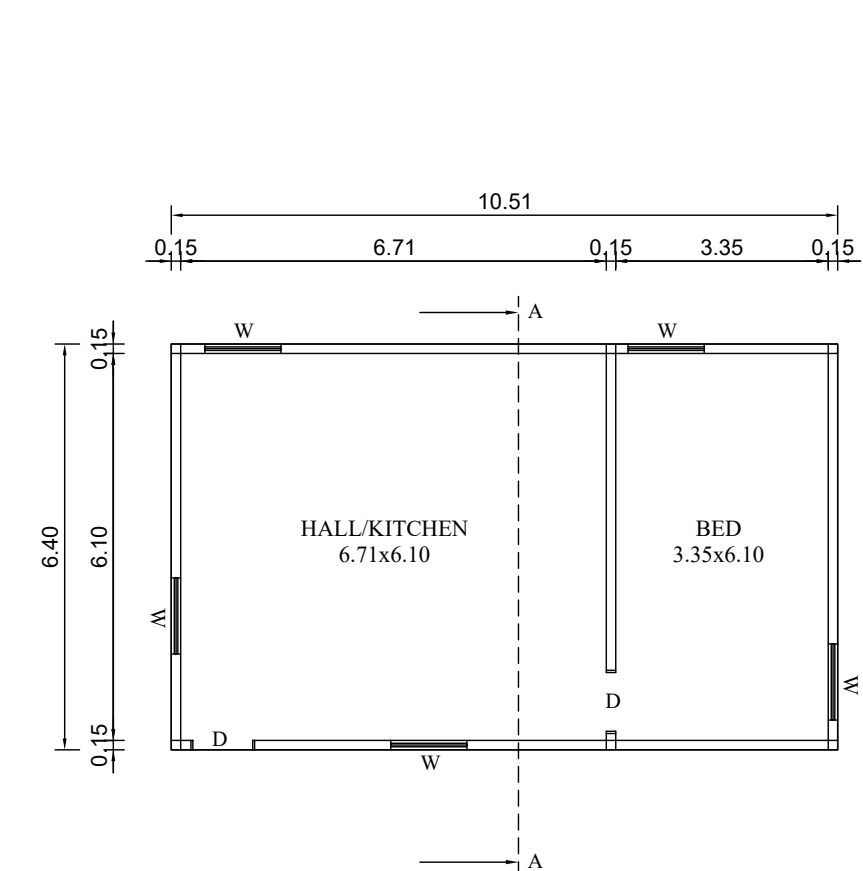
DETAILED PLAN
