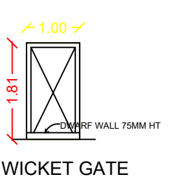
WICKET GATE
