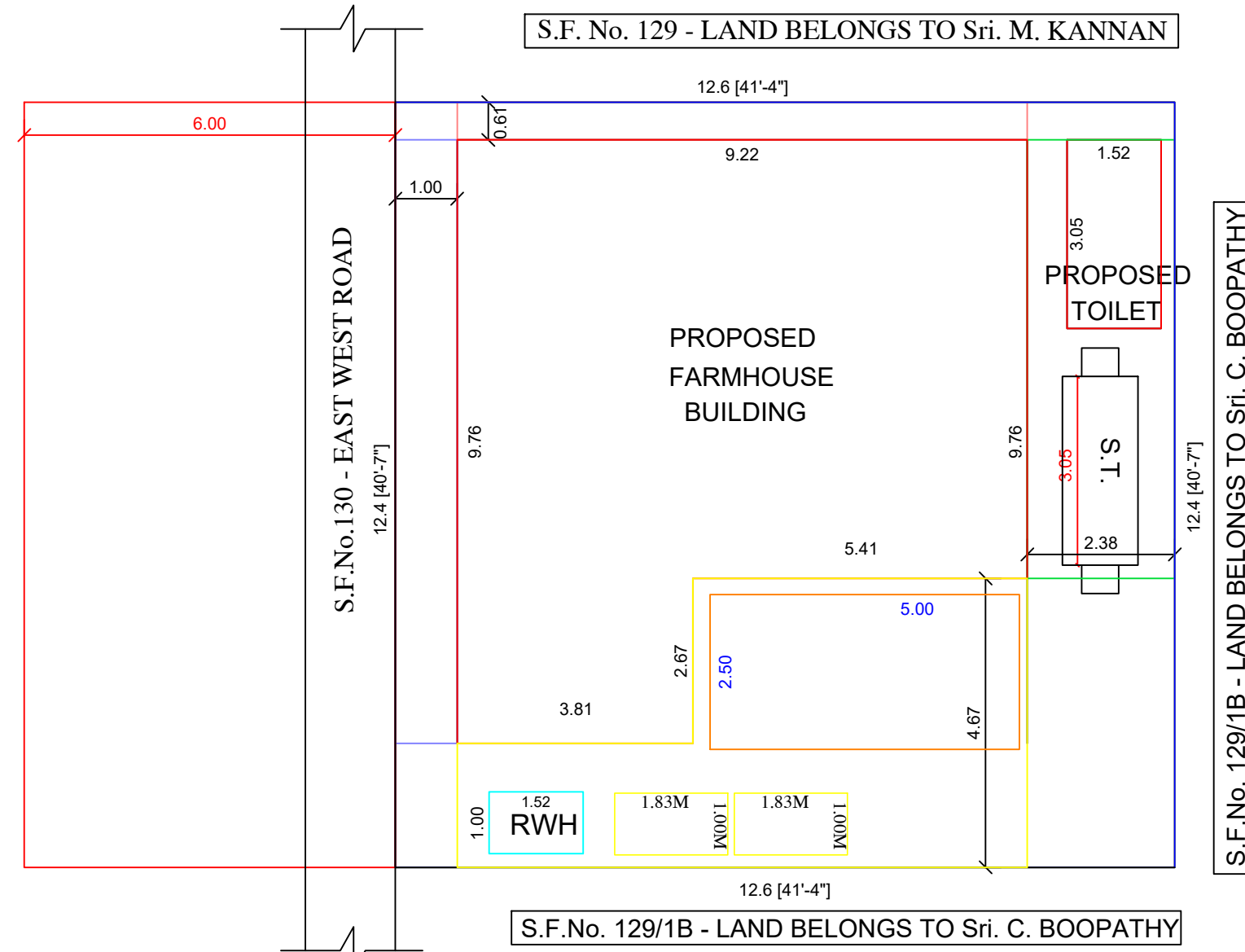
SITE PLAN - MEANT FOR FARM HOUSE
