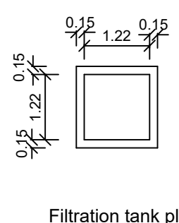
Filtration tank plan
