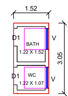
TOILET BLOCK PLAN
