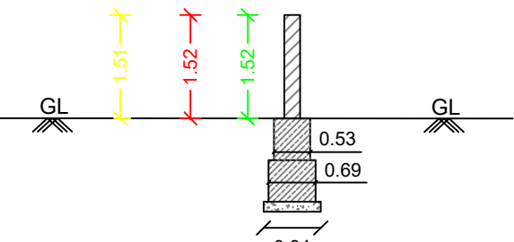
COMPOUND WALL
