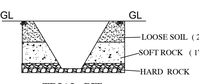
TRIAL PIT
