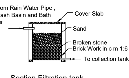
Section Filtration tank
