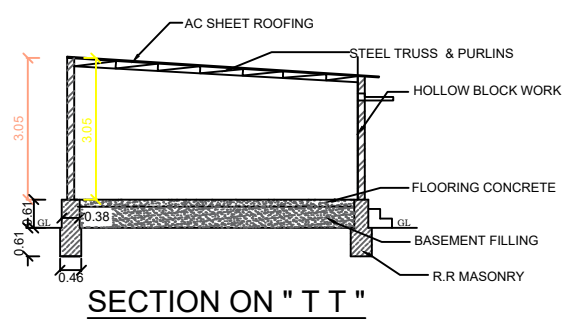
SECTION ON " T T "
