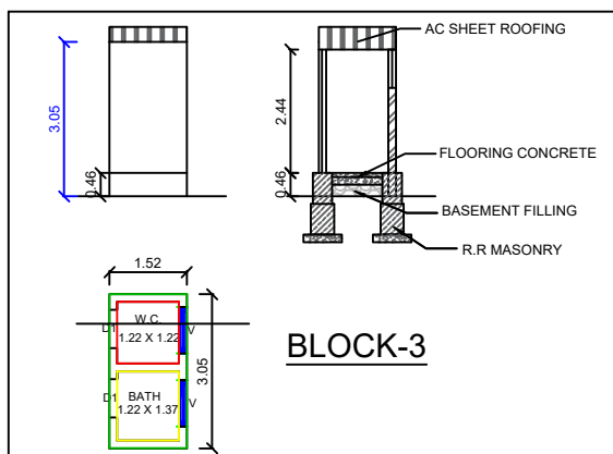
TOILET BLOCK PLAN
