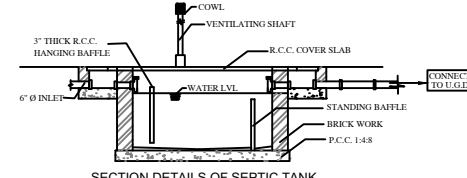
SECTION DETAILS OF SEPTIC TANK
