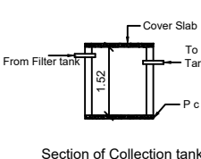
Section of Collection tank
