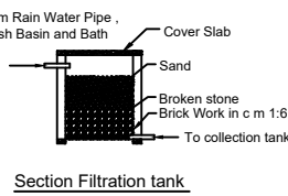
Section Filtration tank
