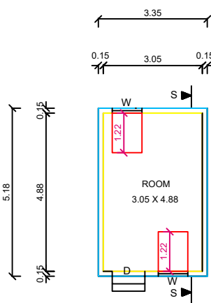
LABOUR QUARTERS PLAN
