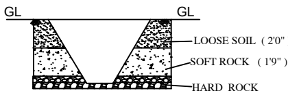
DETAILED PLAN OF RAINWATER PERCUATION AND COLLECTION PIT
