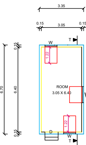
OFFICE PLAN
