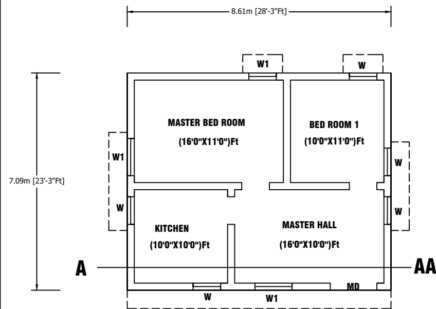
GROUND FLOOR PLAN ON EAST FACE
