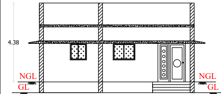
ELEVATION ON EAST FACE
