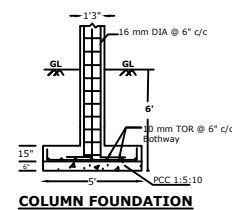
COLUMN FOUNDATION
