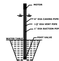
SECTION OF BOREWELL
