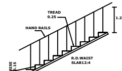
STAIRCASE DETAILS
