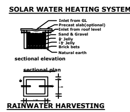
RAINWATER HARVESTING
