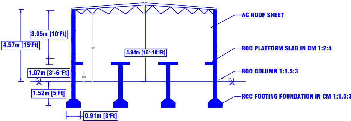
SECTION ON-AA
