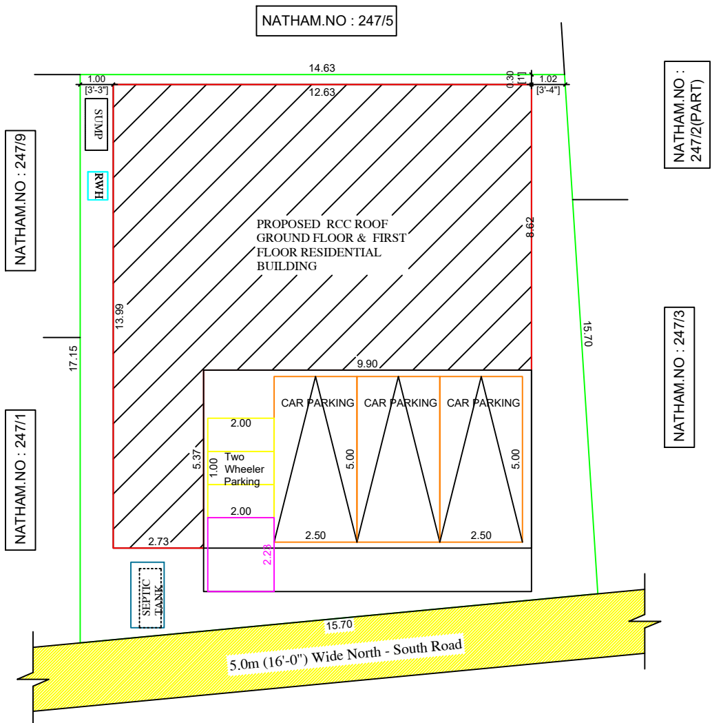
SITE PLAN
