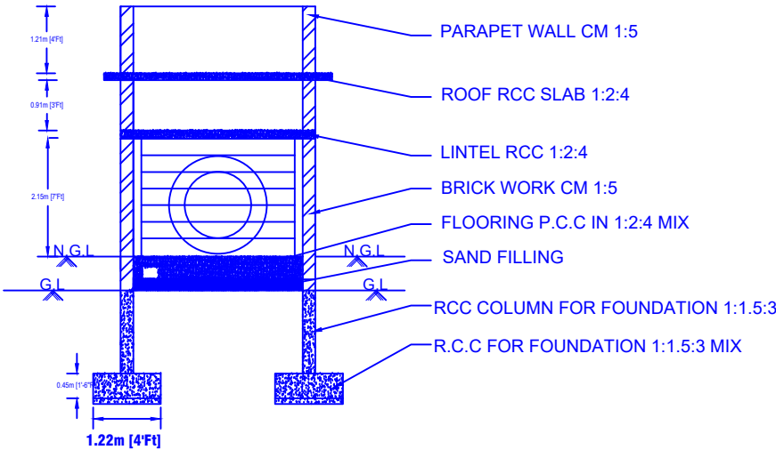
SECTION ON-AA
