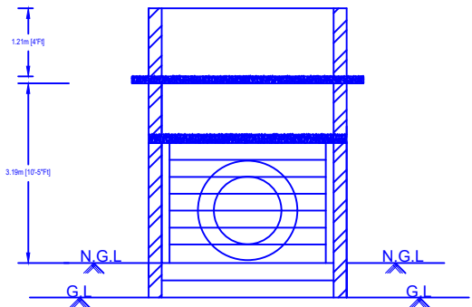
ELEVATION EAST FACING
