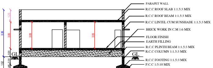
SECTION ON "AB" (SCALE 1: 100)
