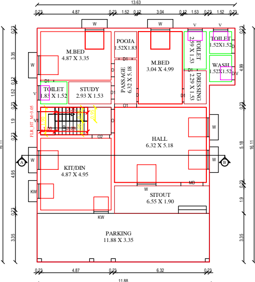
PROPOSED GROUND FLOOR PLAN (SCALE 1: 100)
