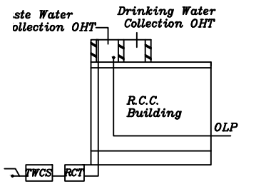
Diagram of Waste Water Recycling & Reuse
