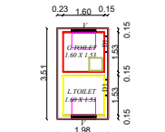
PRO.TOILET PLAN
