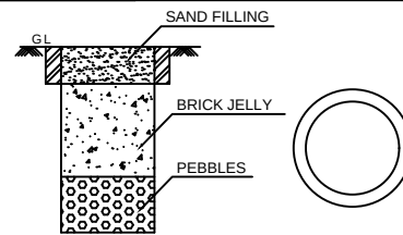
RAIN WATER HARVESTING SYSYTEM
