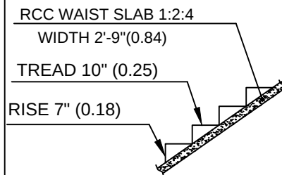
STAIRCASE DETAIL
