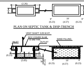
SECTION ON SEPTIC TANK & DISP-TRENCH
