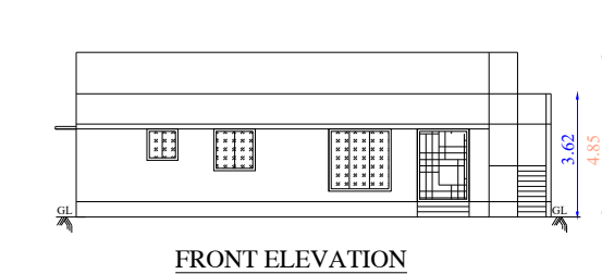
FRONT ELEVATION
