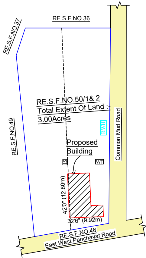
SITE PLAN
