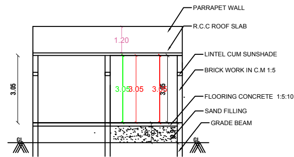
SECTION-AB
