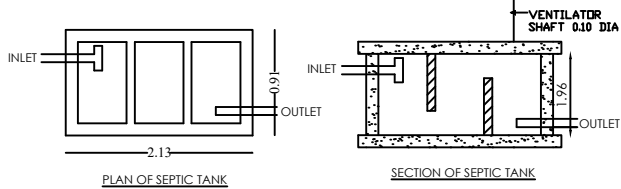
DETAILED DRAWING FOR SEPTIC TANK 225 GALLONS CAPACITY OF 1000 LITRES
