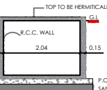
SECTION ON AA
