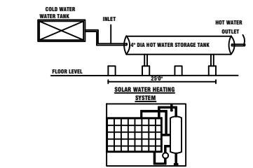
SOLAR HOT WATER SYSTEM DETAILS
