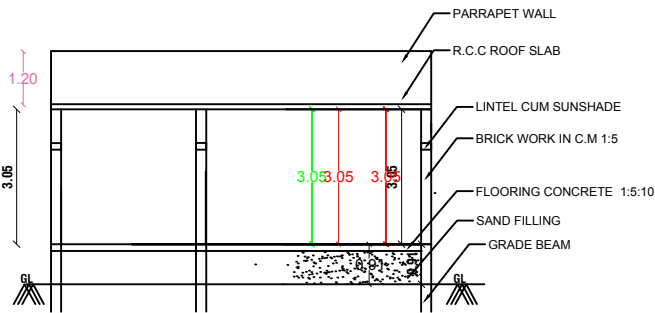
SECTION-AB
