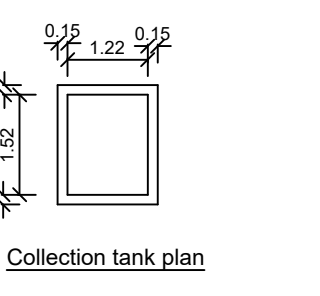
Collection tank plan
