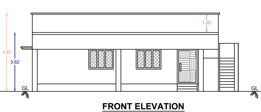
FRONT ELEVATION
