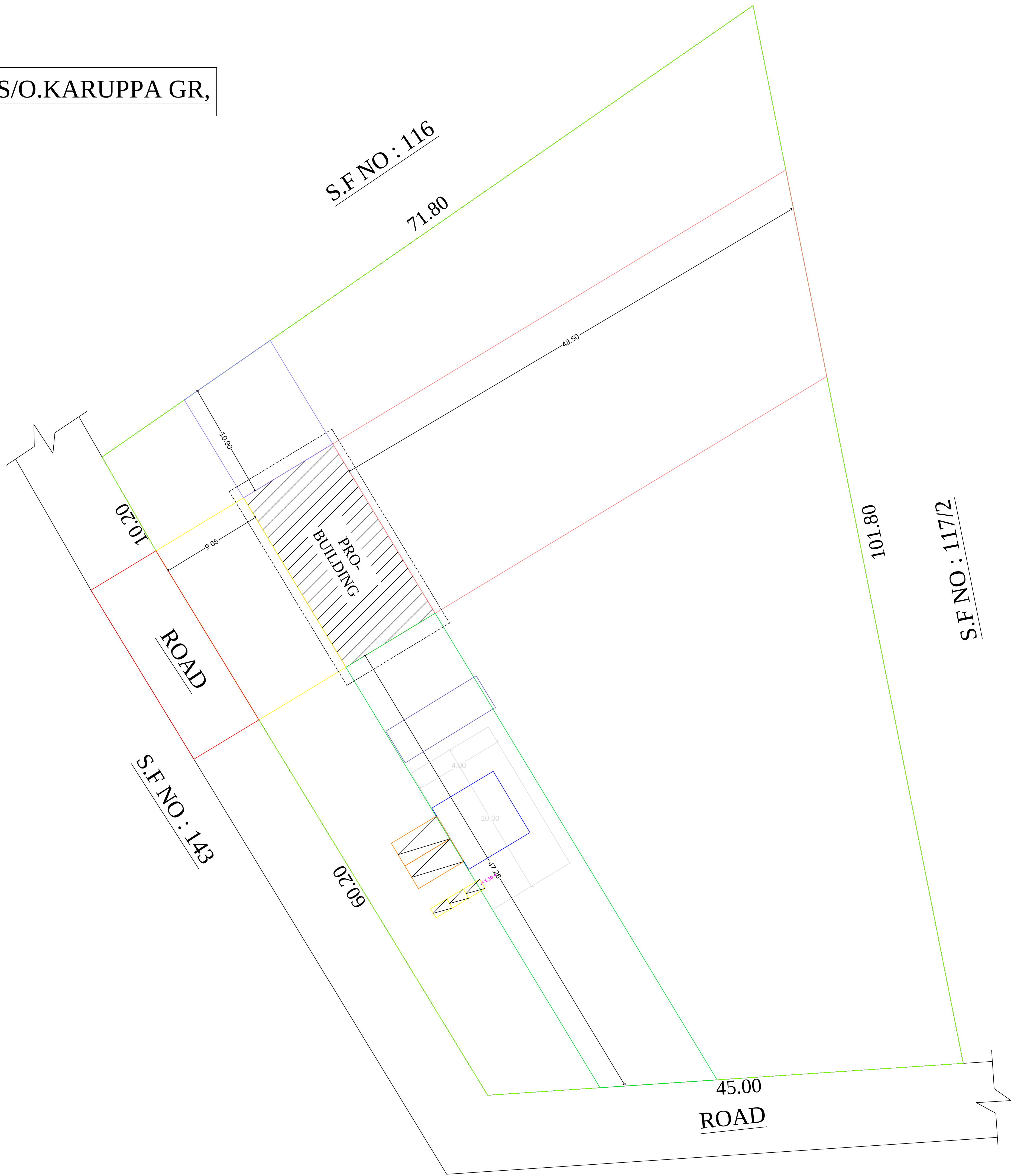
SITE PLAN
