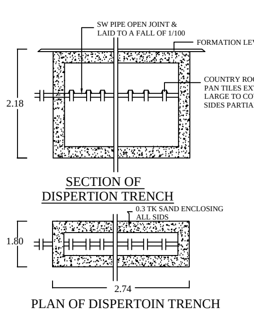
DISPERSION TRENCH
