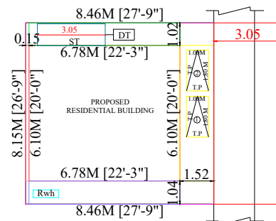
SITE PLAN(MEANT FOR CONSTRUCTION)
