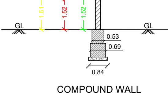
COMPOUND WALL
