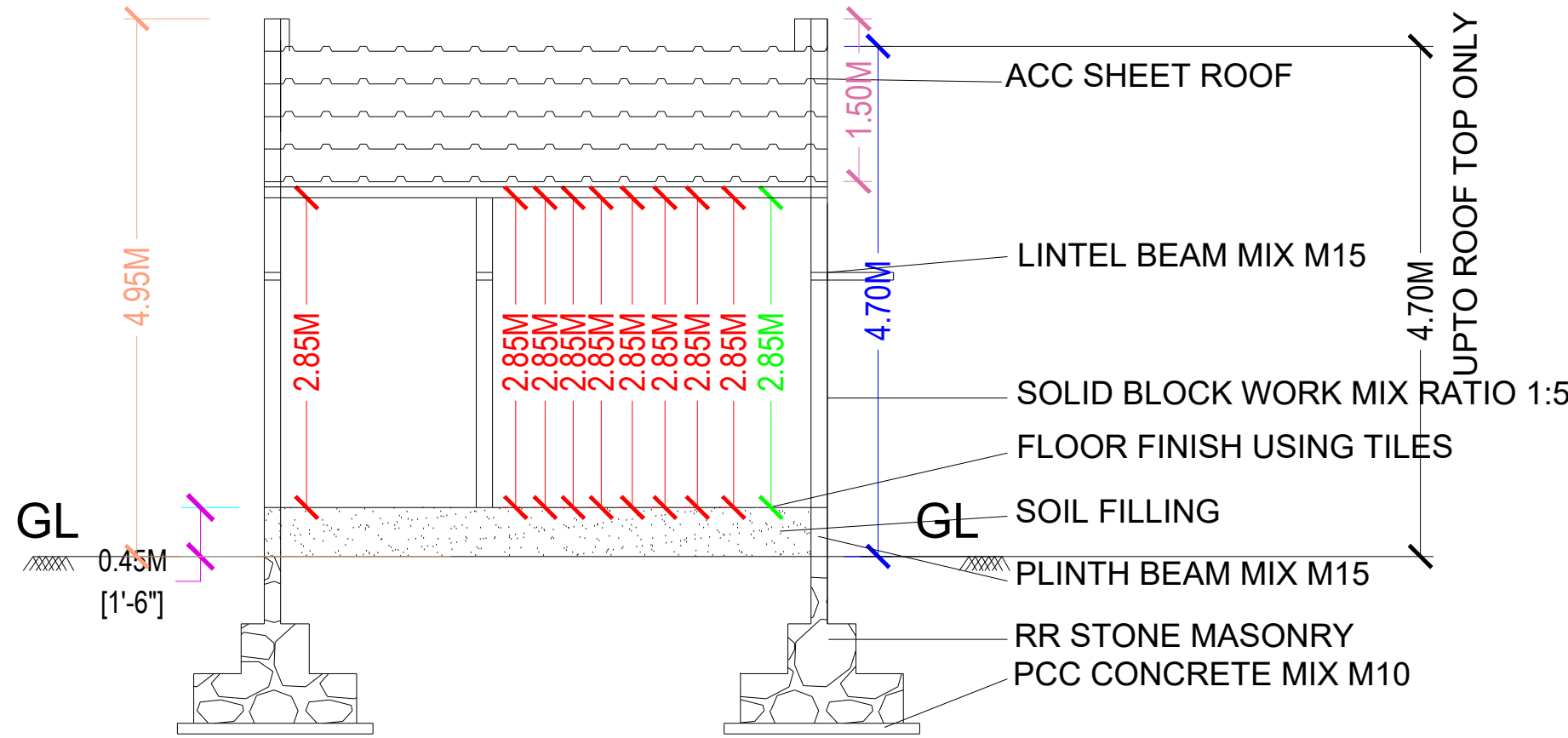
SECTION
