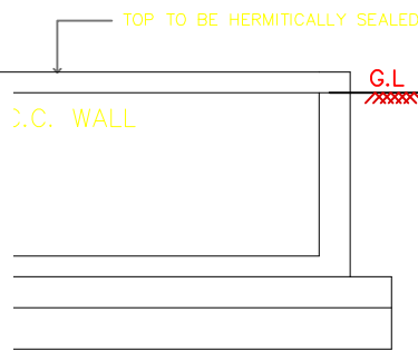
SECTION (SAMPLE)
