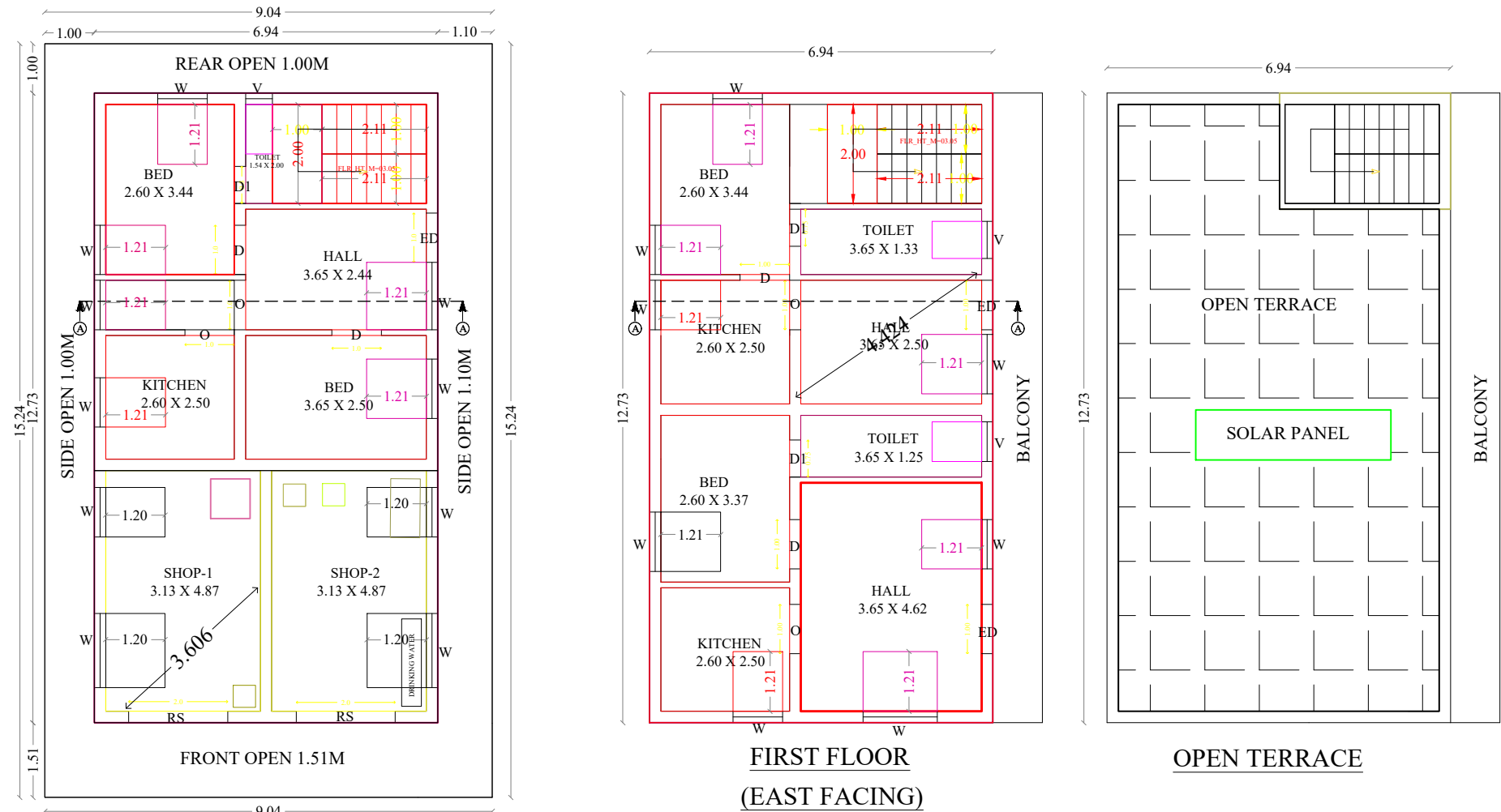
GROUND FLOOR (EAST FACING)
