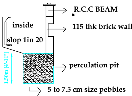
Rain water harvesting plant
