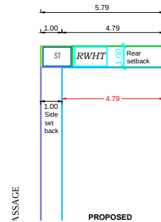
SITE PLAN
