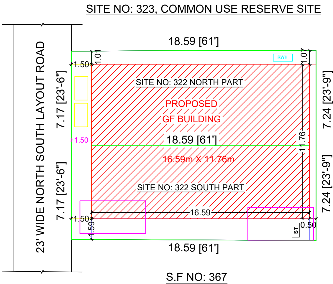
SITE PLAN
