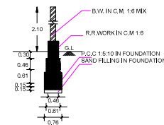
COMPOUND WALL
