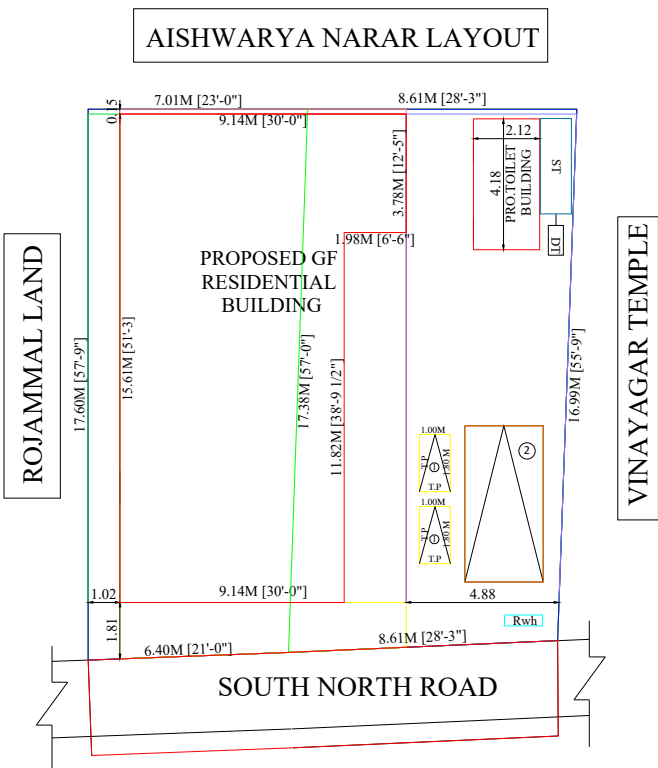
SITE PLAN
