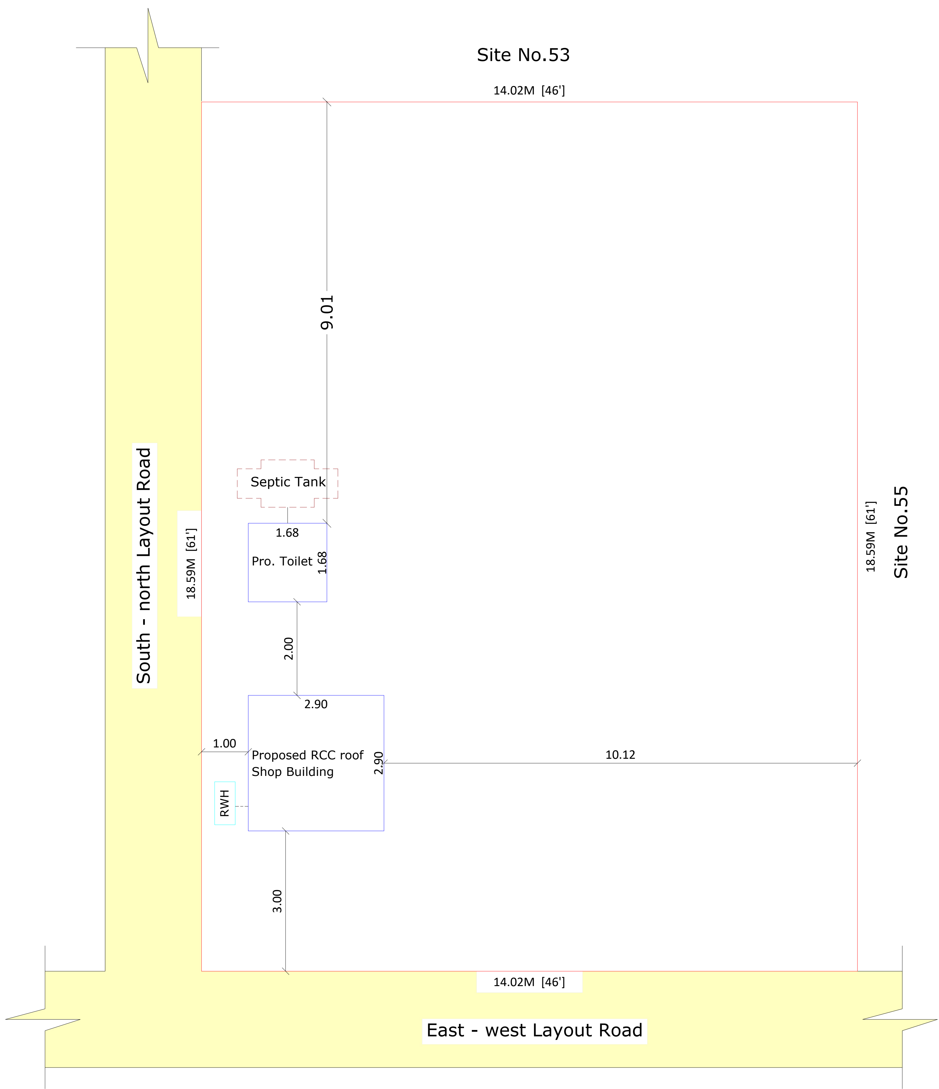
SITE PLAN
