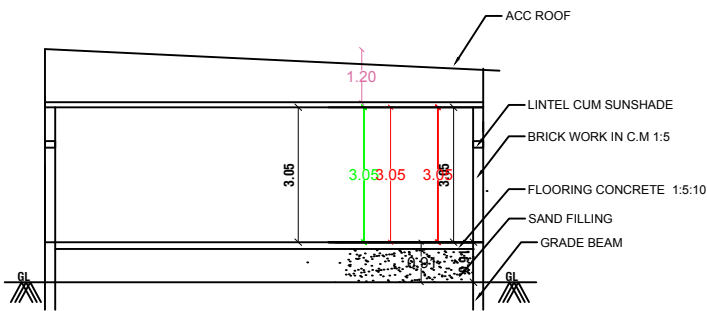
SECTION-AB
