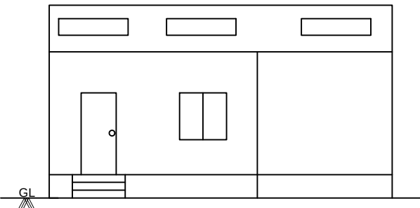
FRONT ELEVATION
