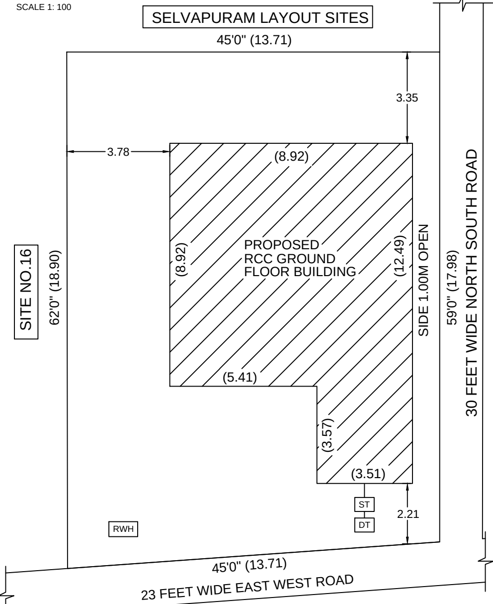
SITE PLAN
