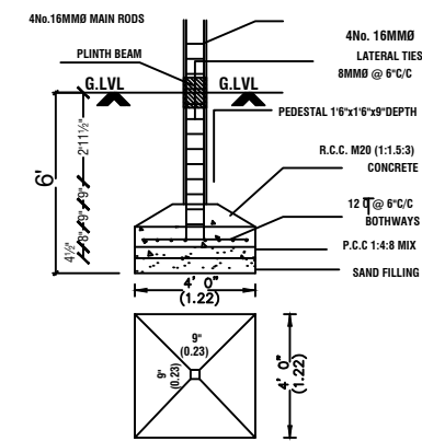
FOUNDATION DETAIL
