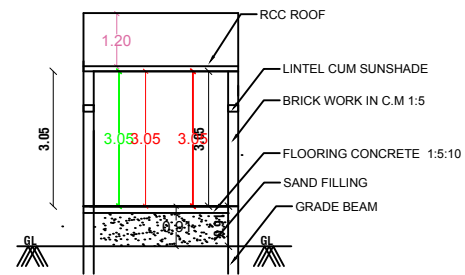
SECTION-AB
