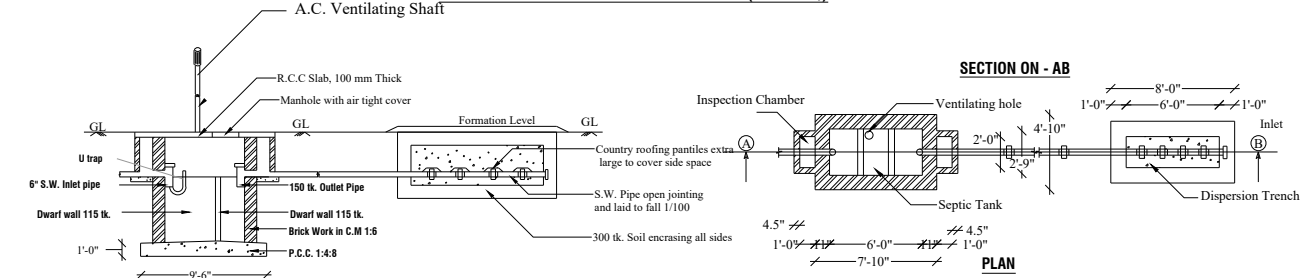
SEPTIC TANK WITH DISPERSION TRENCH ( 250 Gls.,)
