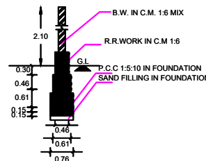
COMPOUND WALL
